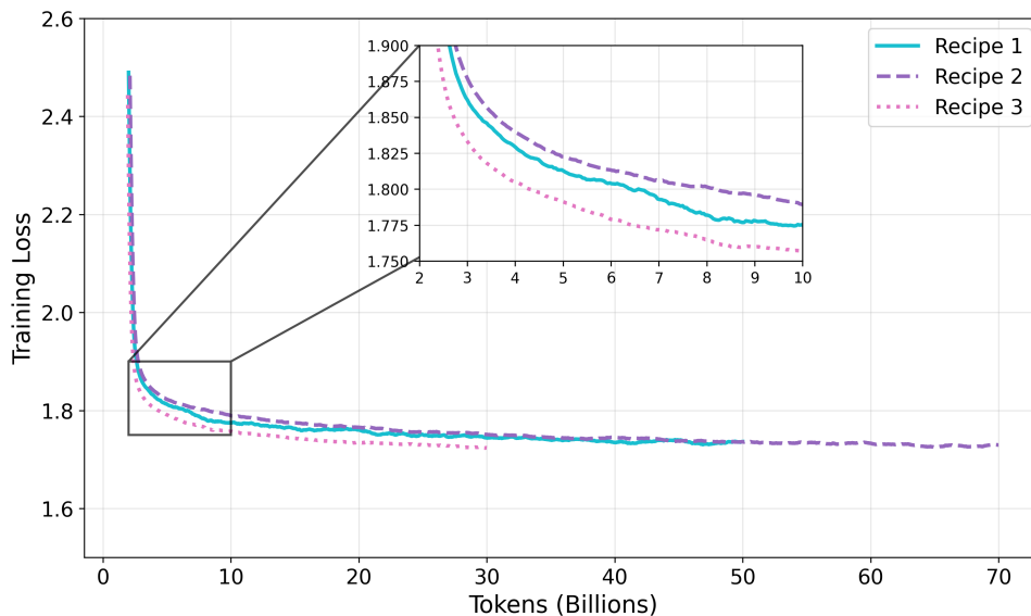
Figure 3: Pre-training loss curves for the three recipes.
