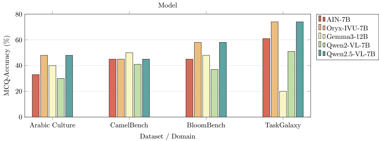
(a) MCQ accuracy (Arabic)
