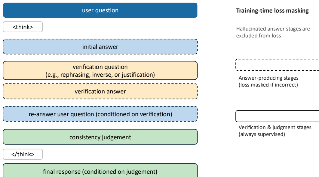
Figure 5: Structured verification trace consisting of an initial answer, a verification question generated through semantic transformations such as rephrasing or logical variation, a verification response, a re-answer conditioned on verification, and a final consistency judgment to determine answer versus abstention. During training, stage-level loss masking suppresses gradients for hallucinated answer-producing stages while preserving supervision for verification and judgment stages.
