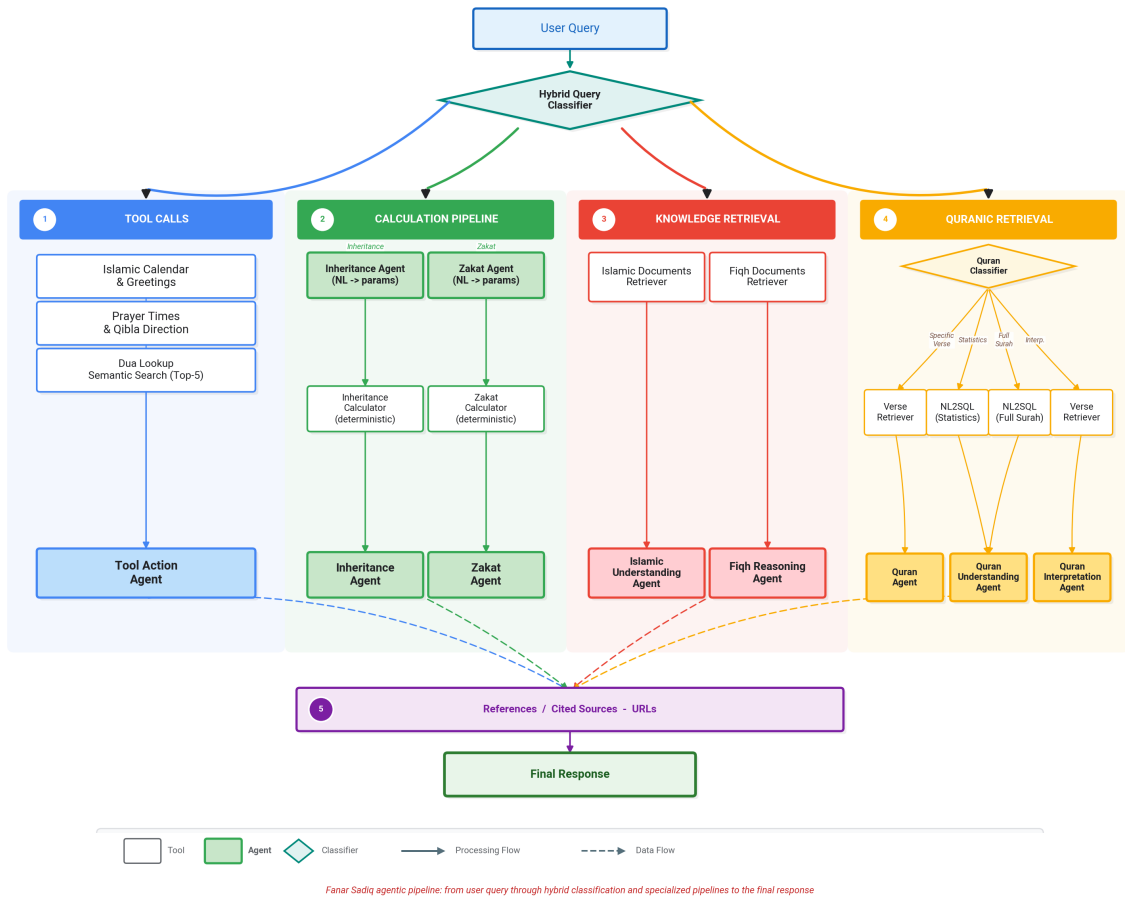
Figure 14: Fanar-Sadiq system pipeline showing hybrid routing, specialized agents, and response verification steps before final answer generation.
