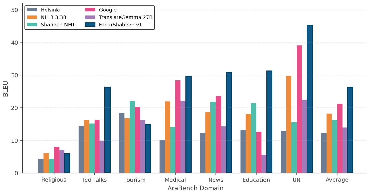
Figure 12: Average BLEU scores for English→Arabic machine translation across AraBench domains. Results are grouped by domain and compare FanarShaheen v1 against open-source, multi-lingual, and commercial MT systems.
