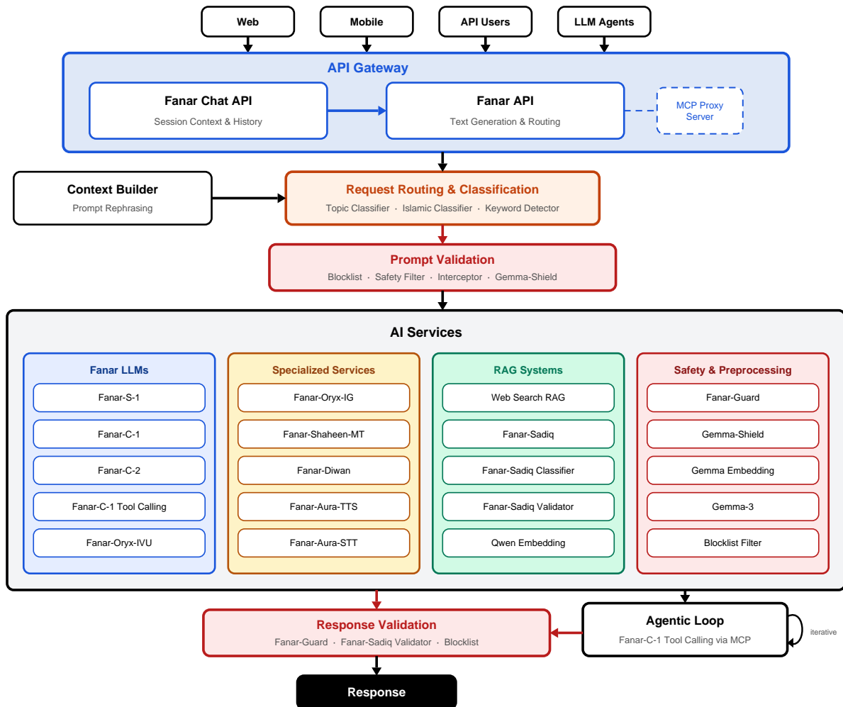
Figure 17: High-level architecture of the Fanar platform showing the orchestrator’s request routing, validation, and service coordination.
