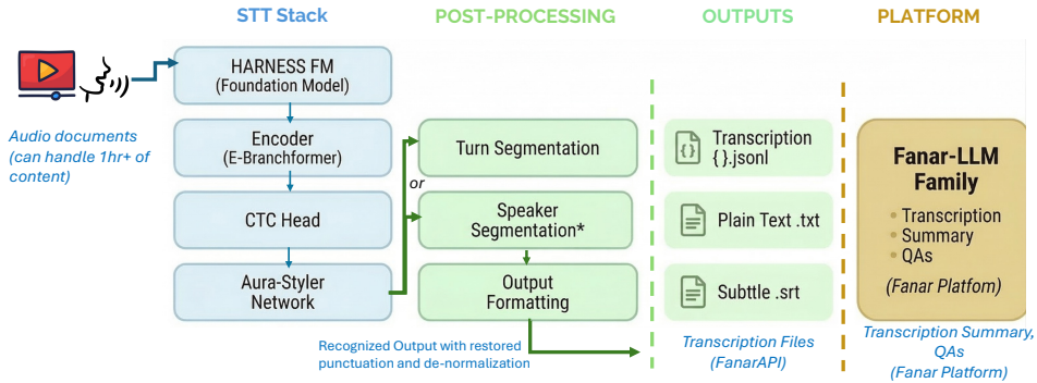
Figure 6: Overview of the Aura-STT-LF long-form speech-to-text model framework, which features long-form ASR, punctuation restoration, Arabic transcript styling (text de-normalization), and turn- and speaker-aware segmentation.
